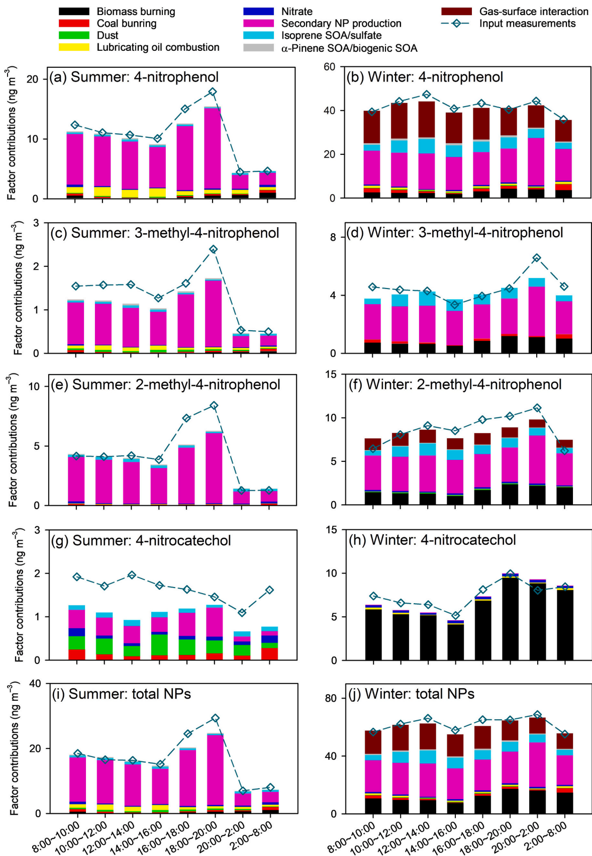
Fig. 4. Diurnal variations of stacked mean factor contributions to individual NPs in PM 2.5 from northern Nanjing in summer (July–August) and winter (January) 2019. The scatter data represent mean values of input measurements.
