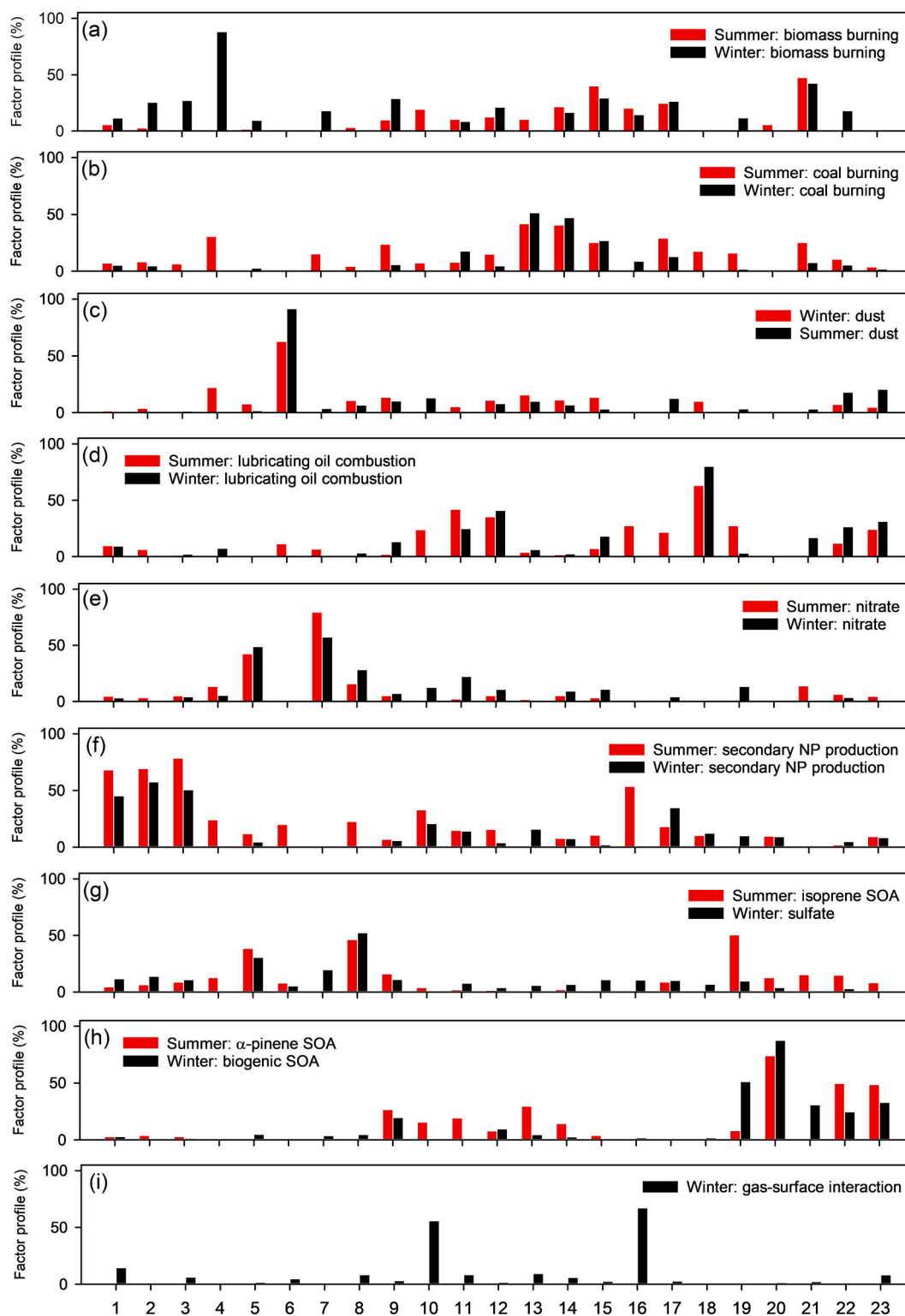
Fig. 3. Comparison of the normalized factor profiles between the 8-factor solution in summer and the 9-factor solution in winter 1. 4-Nitrophenol; 2. 3-Methyl-4-nitrophenol; 3. 2-Methyl-4-nitrophenol; 4. 4-Nitrocatechol; 5. \text{NH}_4^+ ; 6. \text{Ca}^{2+} ; 7. \text{NO}_3^- ; 8. \text{SO}_4^{2-} ; 9. OC; 10. n-Alkanes \lg p_L^{0,*} ( > -8 ); 11. n-Alkanes \lg p_L^{0,*} ( -10 \sim -8 ); 12. n-Alkanes \lg p_L^{0,*} ( < -10 ); 13. PAHs \lg p_L^{0,*} ( > -8 ); 14. PAHs \lg p_L^{0,*} ( -10 \sim -8 ); 15. PAHs \lg p_L^{0,*} ( < -10 ); 16. oxy-PAHs \lg p_L^{0,*} ( > -8 ); 17. oxy-PAHs \lg p_L^{0,*} ( < -8 ); 18. Steranes and hopanes; 19. Isoprene SOA tracers; 20. \alpha -Pinene SOA tracers; 21. Anhydrosugars; 22. Sugar alcohols; 23. Saccharides.
